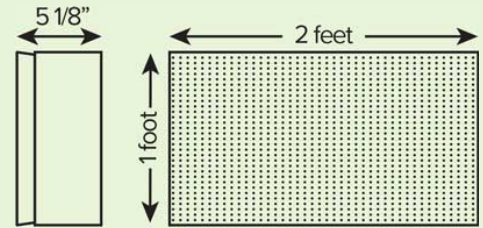
Single LED panel with aluminum frame
